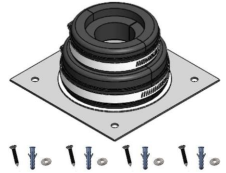
FT-158 for 1-5/8" HELICABLE™ HJA158-50-A Air-Dielectric Coaxial Cable
