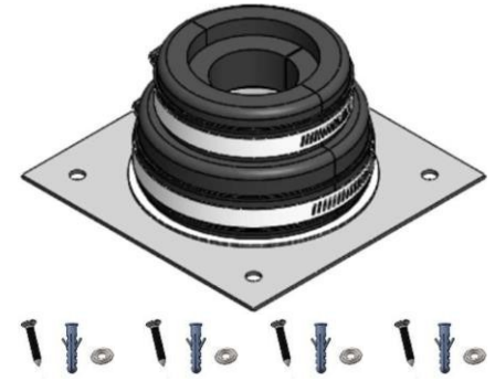
FT-78 for 7/8" HELICABLE™ HJA78-50-A Air-Dielectric Coaxial Cable
